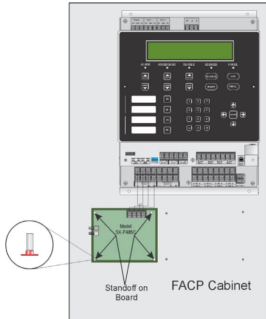
SK-F485C MOUNTING IN FACP CABINET
